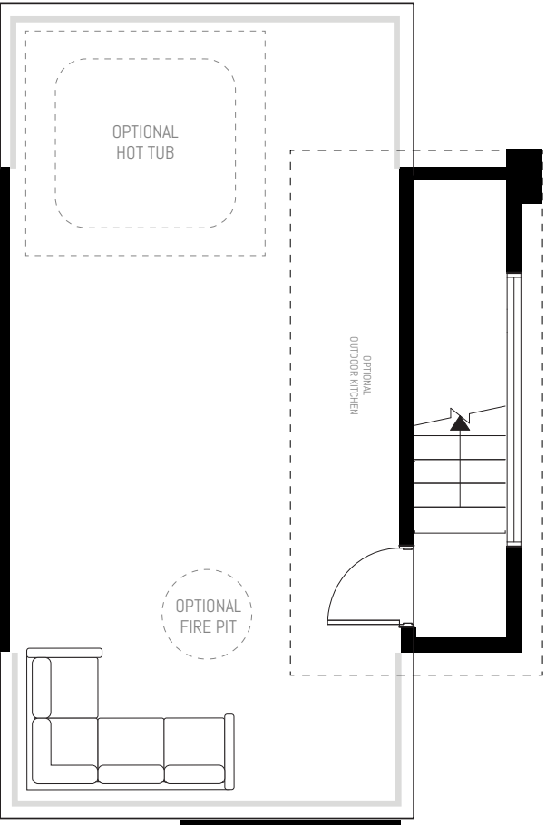
ROOF DECK
