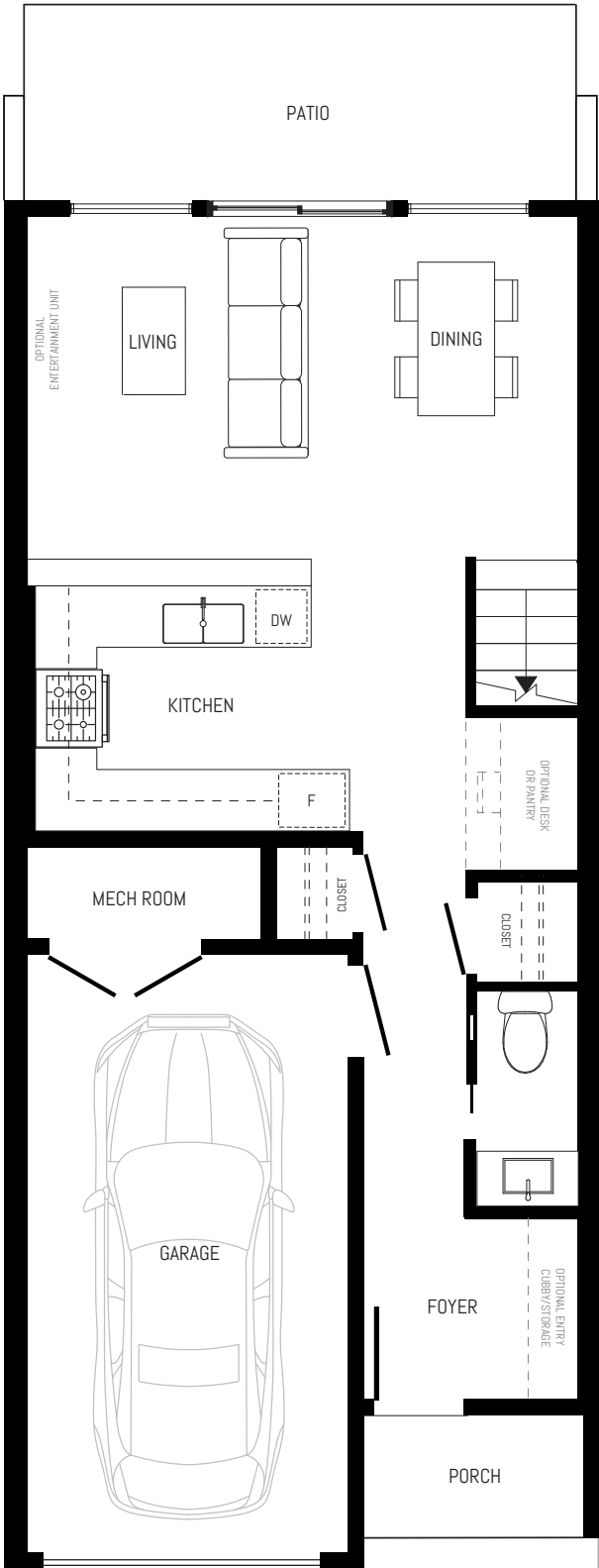
MAIN FLOOR
