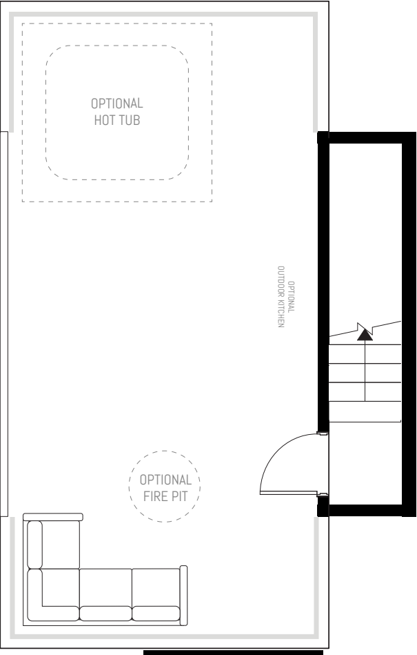
ROOF DECK
