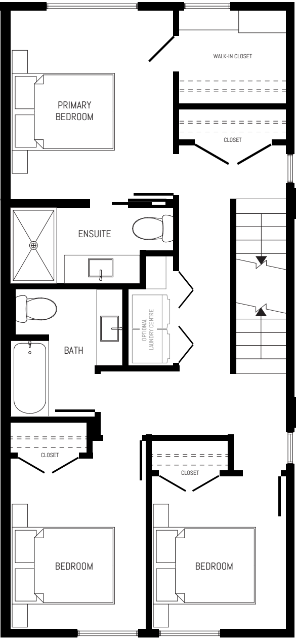
UPPER FLOOR
