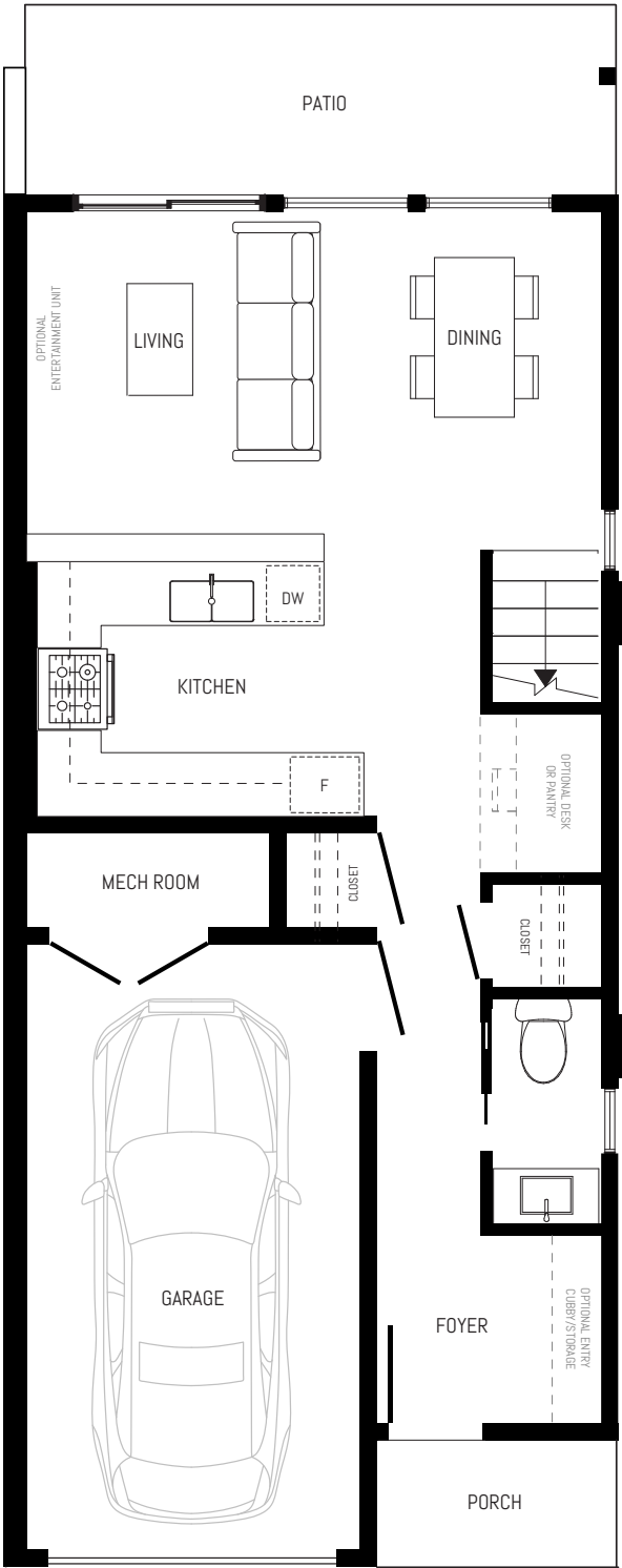
MAIN FLOOR
