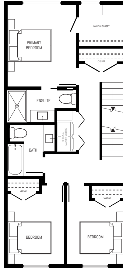
UPPER FLOOR
