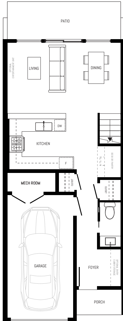
MAIN FLOOR
