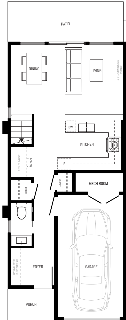
MAIN FLOOR
